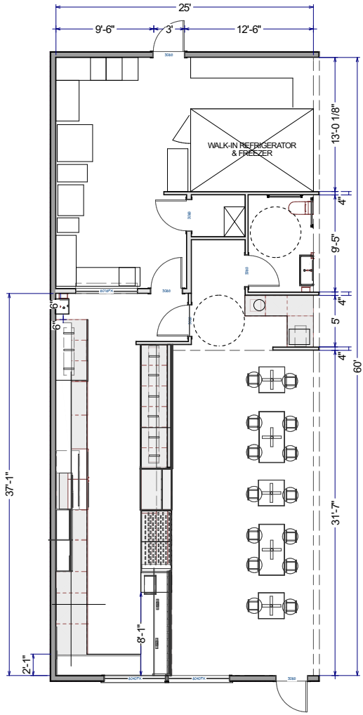
PROPOSED FLOOR PLAN SCALE: 1/4" = 1'0"
